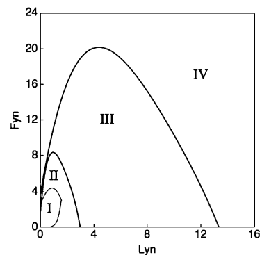
FIGURE 6. Dependence of BCR signaling dynamics on Lyn and Fyn copy numbers. Responses to an Ag signal were systematically simulated for different combinations of Lyn and Fyn copy numbers. The Ag signal was a step increase in c to 3. In all cases, the initial state was the basal steady state with c = 0 . Each numbered region in this plot corresponds to one of four qualitative responses seen in simulations. These responses to the Ag signal are (I) no Syk activation, (II) a single pulse of Syk activation, (III) repeated pulses of Syk activation, and (IV) sustained Syk activation, as in Fig. 2B. Note that a value of 1 on either the horizontal or vertical axis corresponds to 10^5 molecules/cell.
