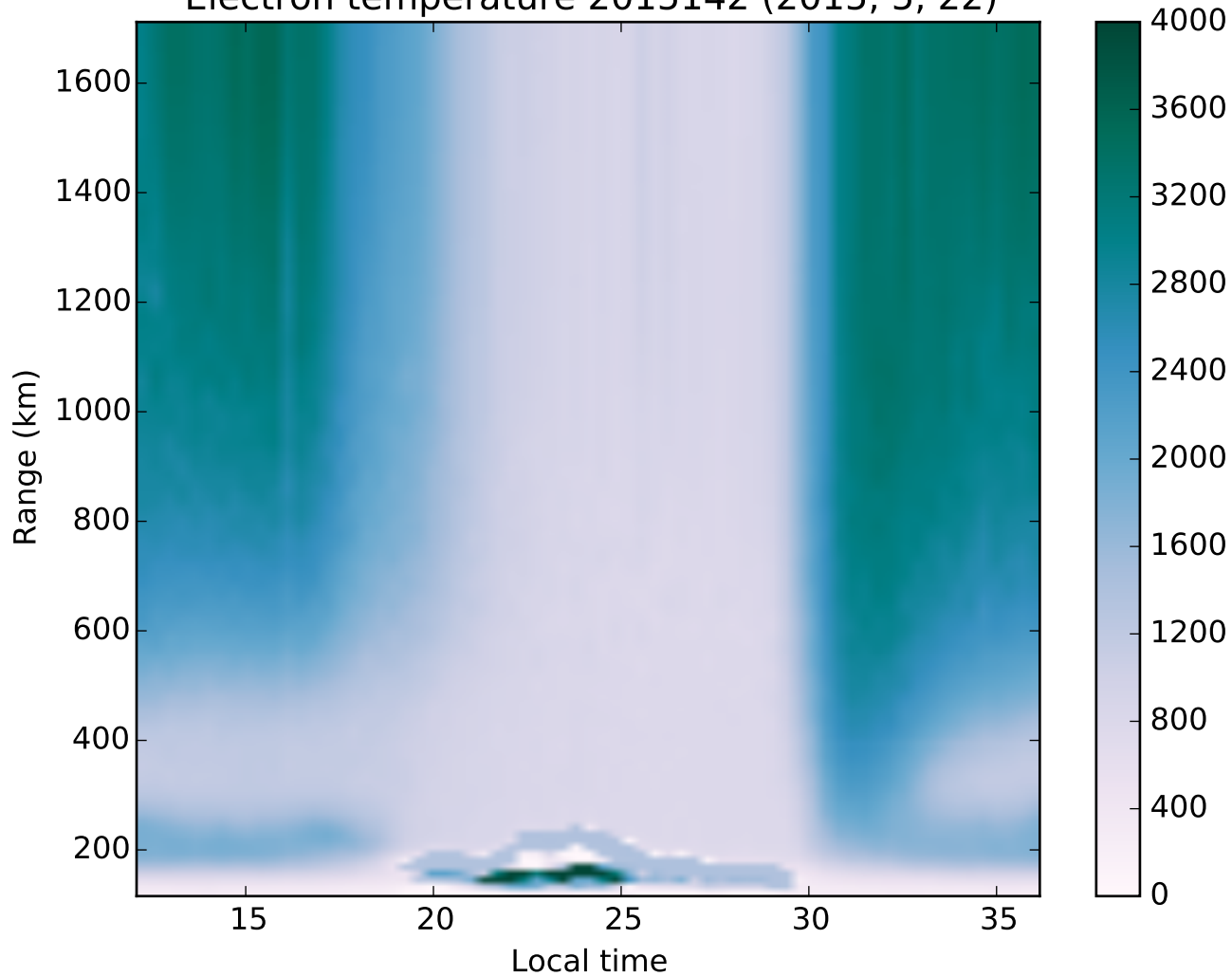
Electron temperature 2015142 (2015, 5, 22)
