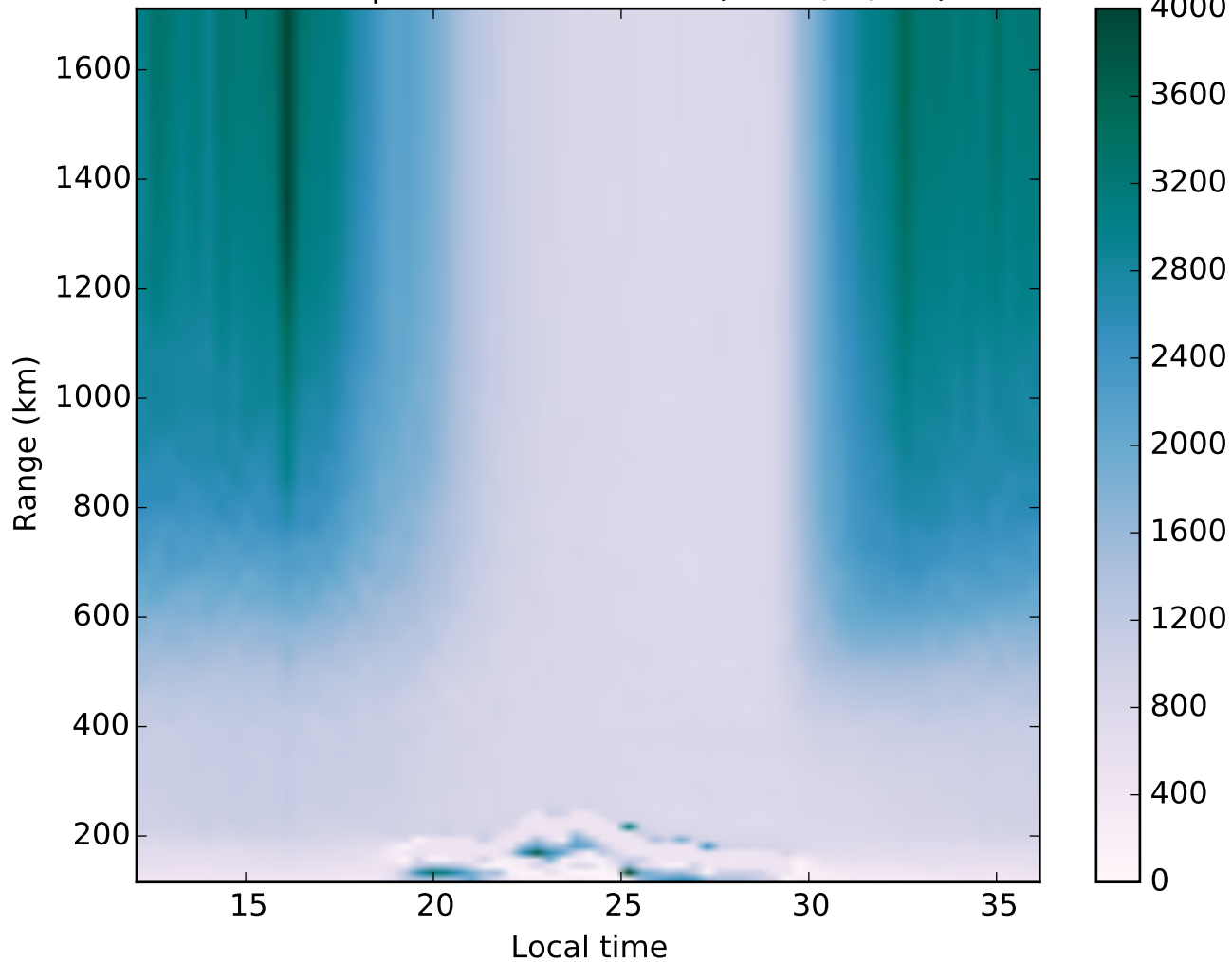
Ion temperature 2015142 (2015, 5, 22)
