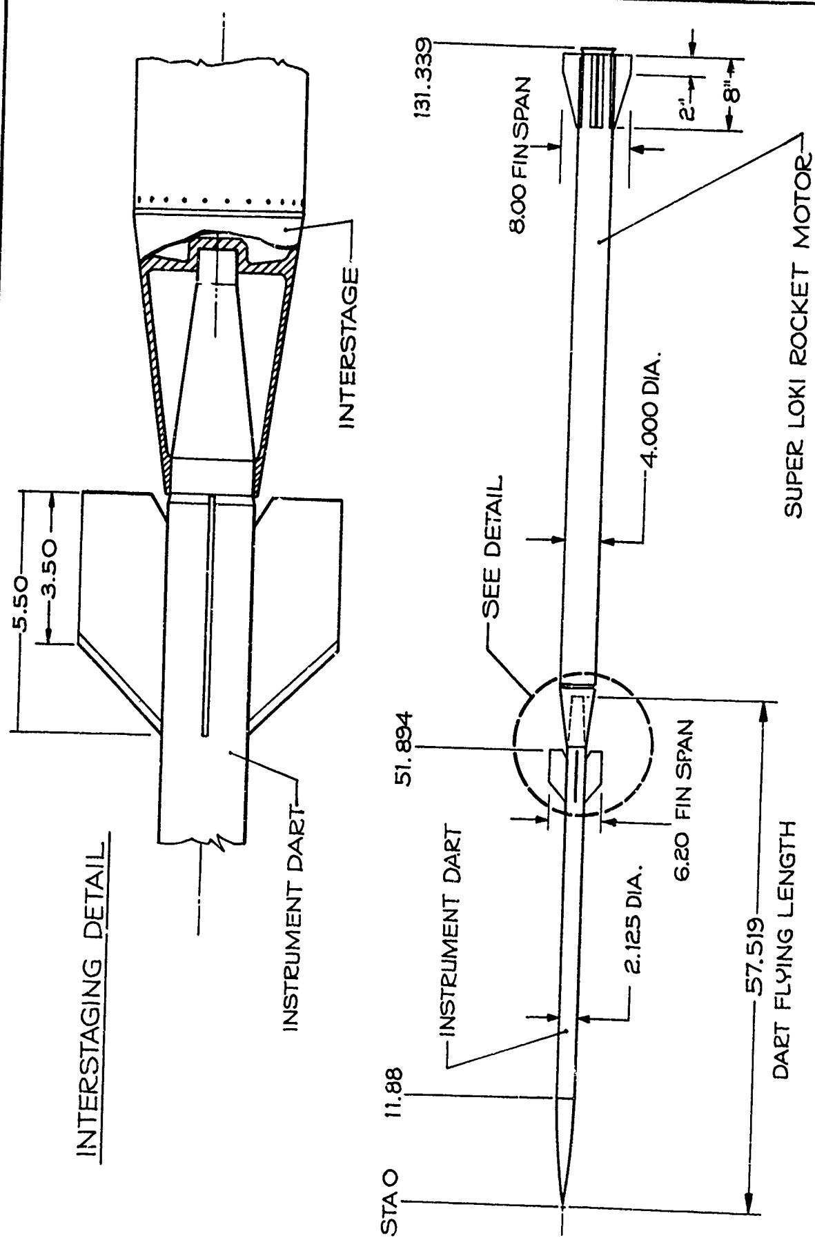
FIGURE 5.3 SUPER LOKI INSTRUMENT DART VEHICLE CONFIGURATION
