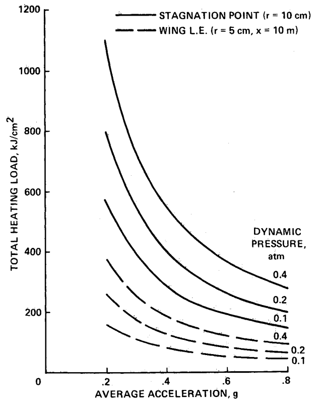
Fig. 7 Ascent total heat loads.
