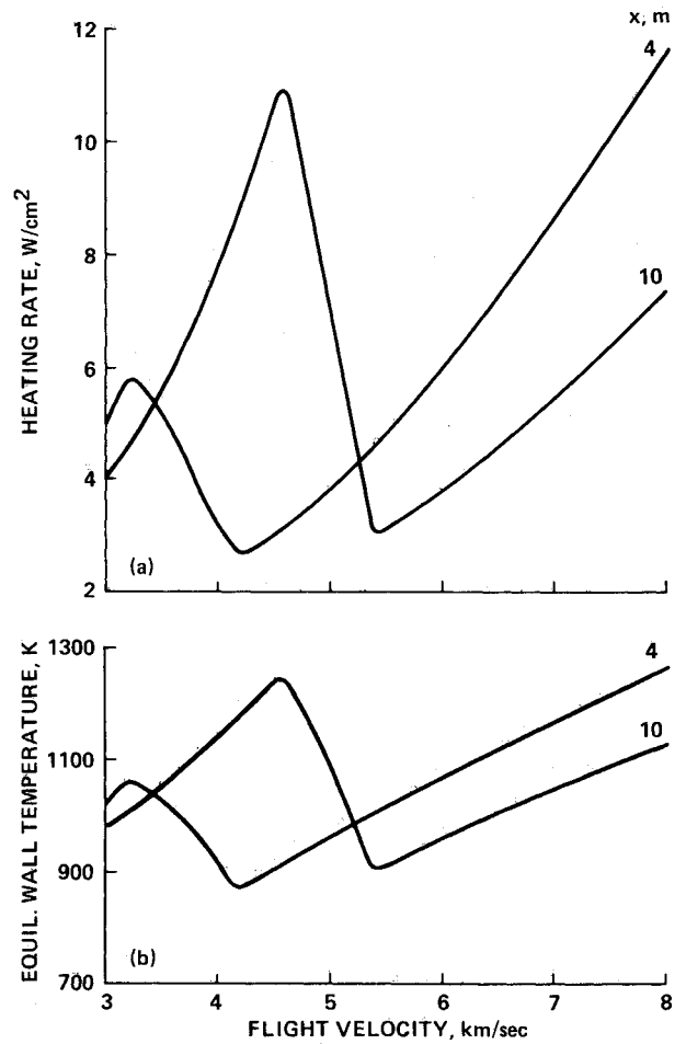
Fig. 6 Body centerline heating during ascent, dynamic pressure = 0.4 atm.
