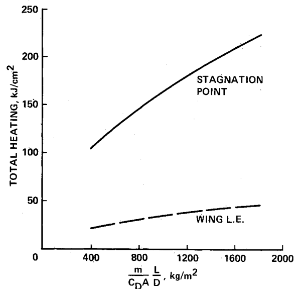
Fig. 11 Total heat loads during entry.
