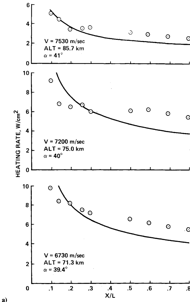
Fig. 2 Comparison of centerline heating calculations with flight data: a) STS-2, b) STS-1.
