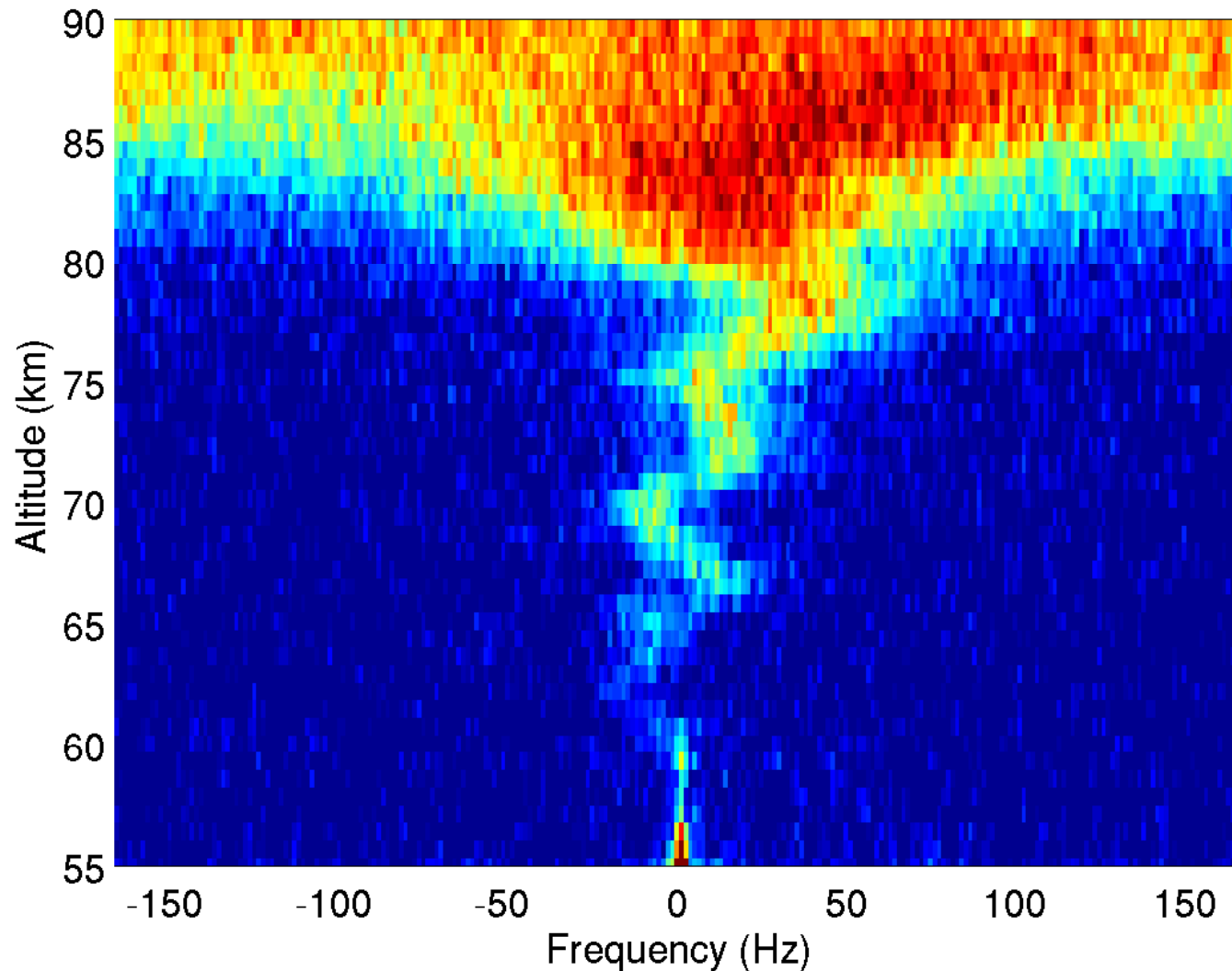
Typical D-region Spectra
