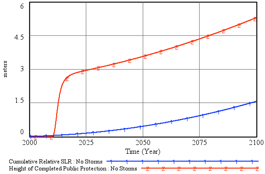
Figure 5-21: The path of RSLR and the height of the protective dune for the example Reference scenario for Miami-Dade County.
