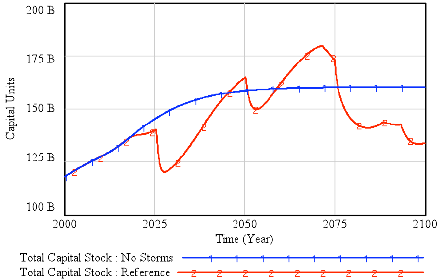
Figure 5-6: Behavior of total capital for the example Reference scenario for Miami-Dade County—the sum of all four capital stocks.
