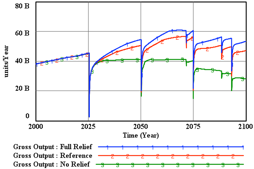
Figure 7-3: Gross output for the disaster relief scenarios. Behavior is for Miami-Dade County over time, given three different levels of government disaster relief.
