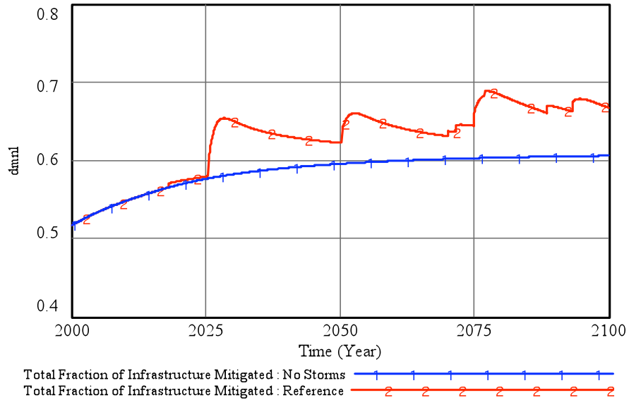
Figure 5-23: The fraction of mitigated infrastructure for the example Reference scenario for Miami-Dade County.
