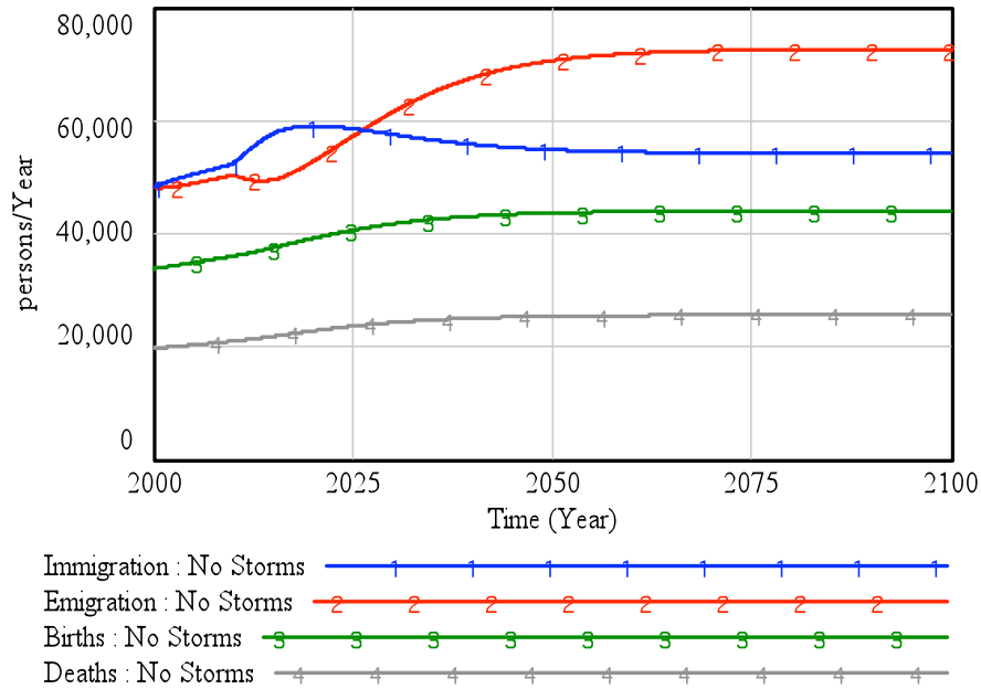
Figure 5-16: Behavior of immigration, emigration, births, and deaths for the No Storms scenario.
