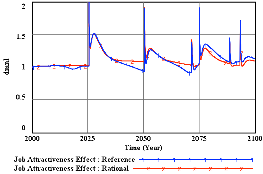
Figure 6-13: The job attractiveness for the rationality scenarios (example pattern for Miami-Dade).
