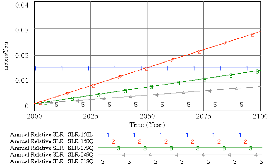
Figure 3-5: Annual RSLR for five global SLR scenarios for Miami-Dade County.
