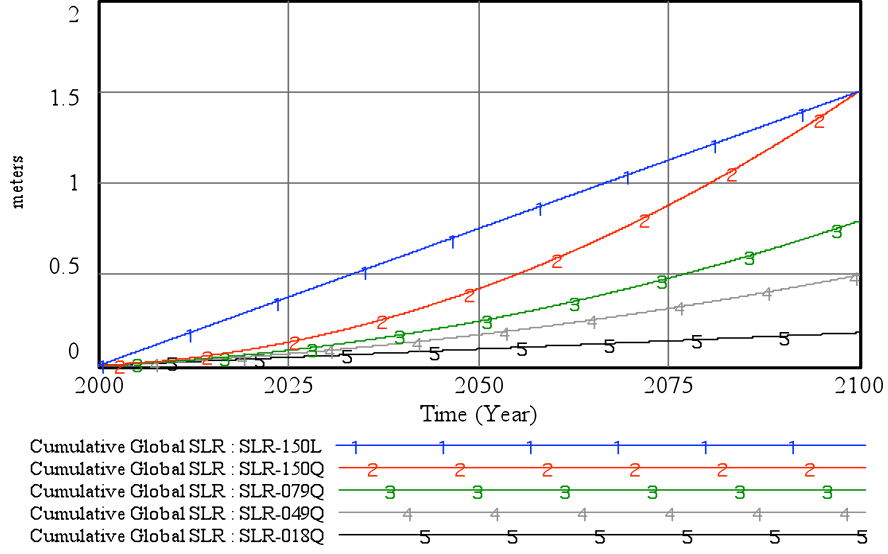
Figure 3-3: Comparison of five different global sea-level rise scenarios.
