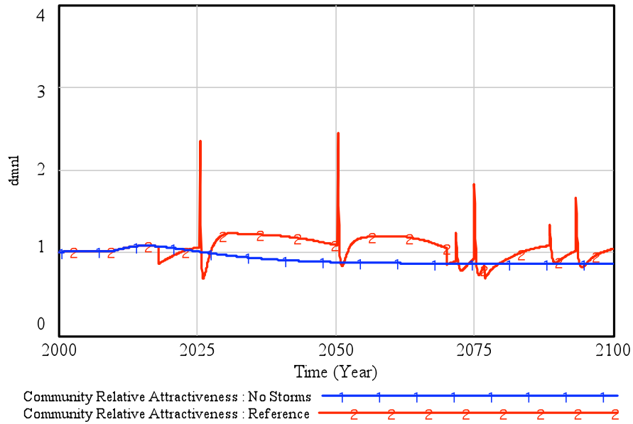
Figure 5-17: Behavior of Community Attractiveness for the example Reference scenario for Miami-Dade County.
