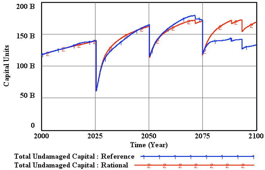
Figure 6-7: Total Undamaged Capital for the rationality scenarios (example pattern for Miami-Dade).
