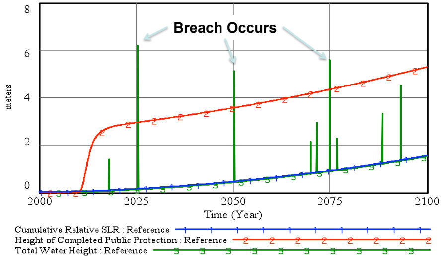
Figure 5-22: The path of RSLR and the height of the protective dune, with total water height during storms, for the example Reference scenario for Miami-Dade County.
