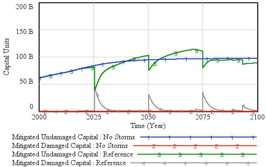
Figure 5-9: Behavior of the mitigated capital stocks for the example Reference scenario for Miami-Dade County.
