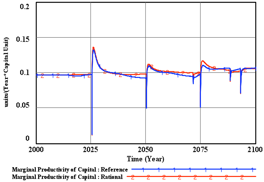
Figure 6-5: The Marginal Productivity of Capital for the rationality scenarios (example pattern for Miami-Dade).
