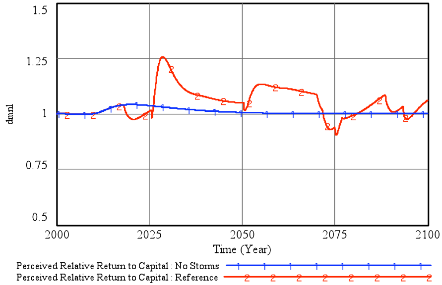
Figure 5-7: The behavior of Perceived Relative Return to Capital for the example Reference scenario for Miami-Dade County.
