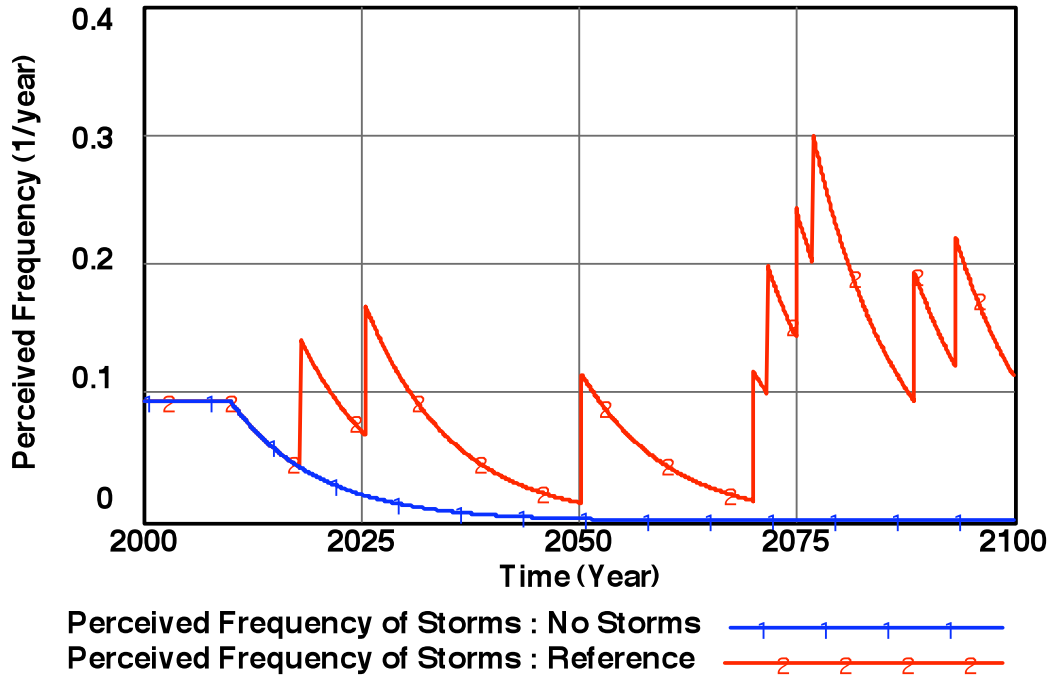
Figure 5-3: The response of Perceived Frequency of Storms to an sample storm pattern of the Reference scenario and a No Storms scenario, for the for Miami-Dade County.
