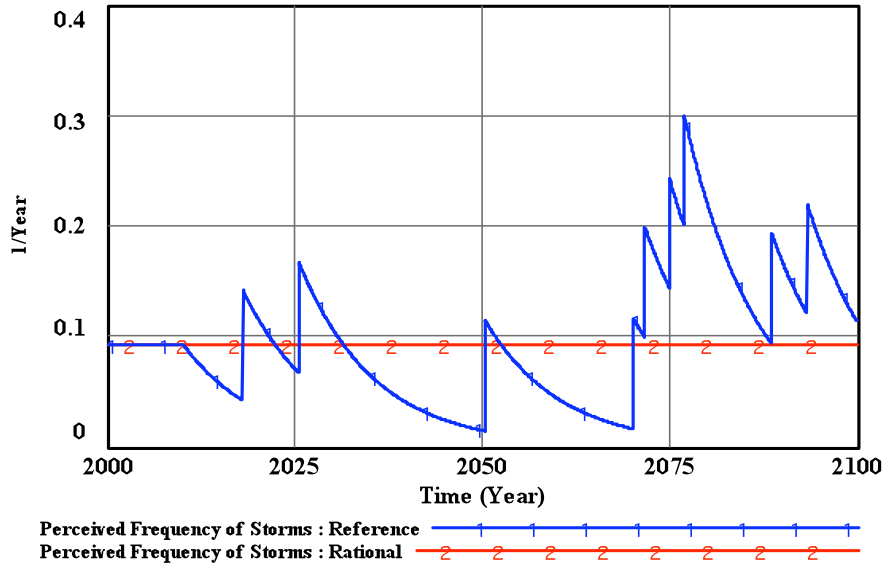
Figure 6-1: The Perceived Frequency of Storms for the rationality scenarios (example pattern for Miami-Dade).
