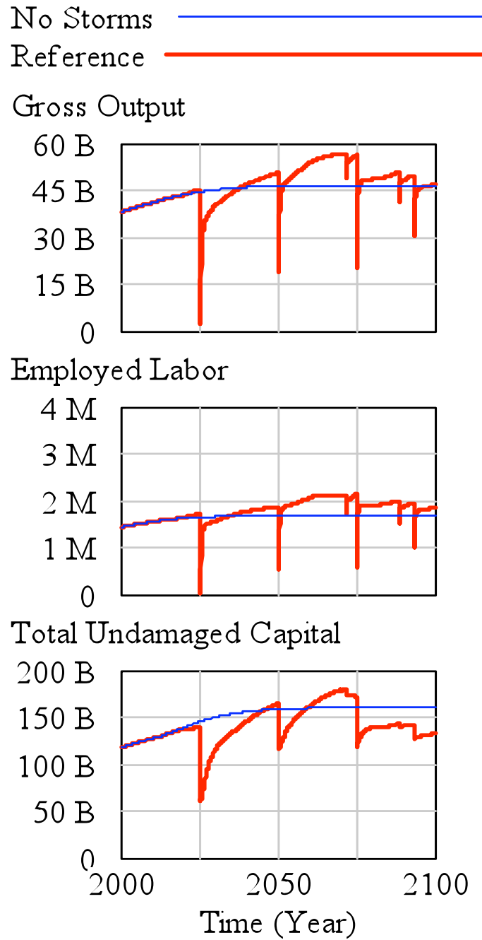
Figure 5-5: Gross Output and the behavior of the two factors of production for the example Reference scenario for Miami-Dade County.
