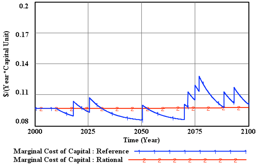
Figure 6-6: The Marginal Cost of Capital for the rationality scenarios (example pattern for Miami-Dade).
