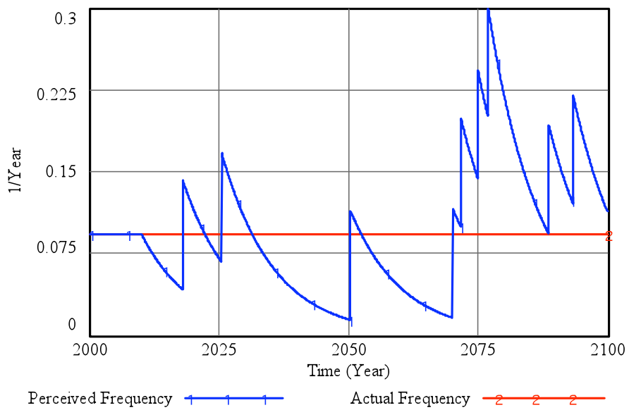
Figure 3-7: Example of perceived storm frequency behavior for a series of storms, compared to the constant actual frequency.
