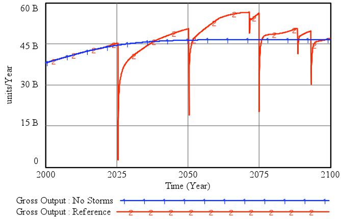
Figure 5-25: Behavior of gross economic output for Miami-Dade.
