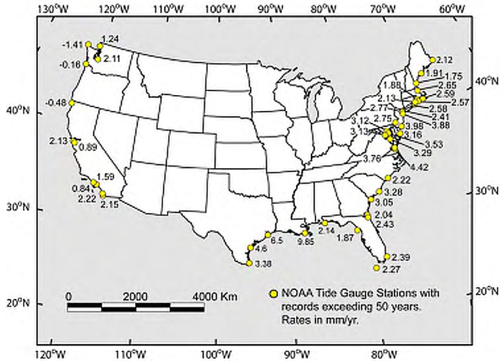
Figure 2-1: Rates of relative sea-level rise around the United States. (Sources: Figure 1.4 from CCSP (2009); Data from Zervas (2001))
