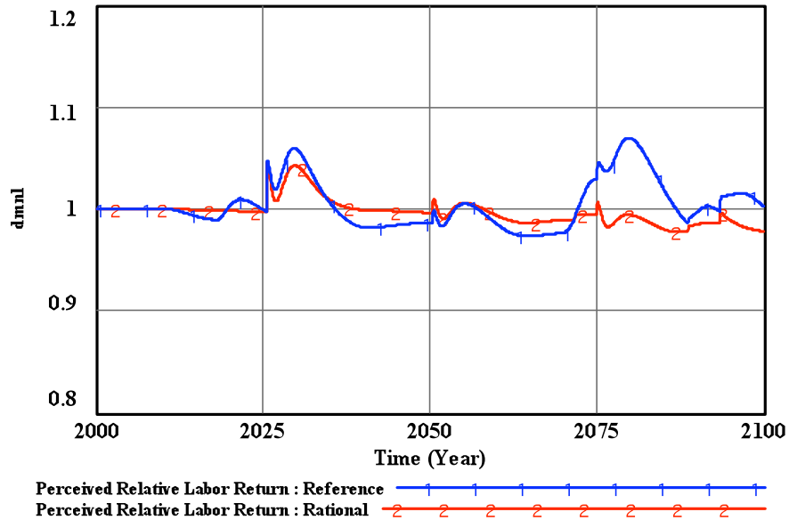
Figure 6-14: The Perceived Relative Return to Labor for the rationality scenarios (example pattern for Miami-Dade).
