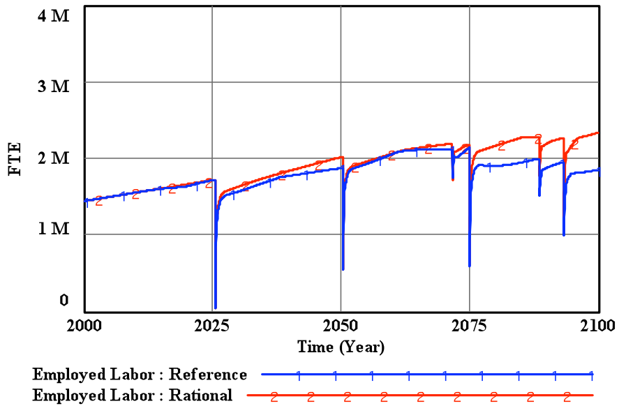
Figure 6-8: Employed Labor for the rationality scenarios (example pattern for Miami-Dade).
