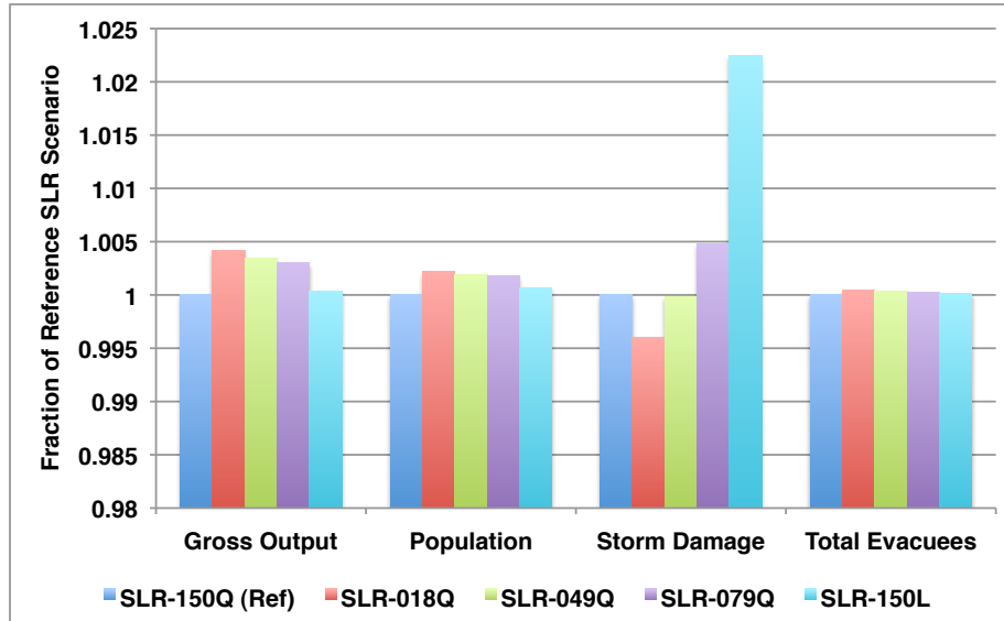
Figure 6-17: Comparison of four metrics for different SLR scenarios. Results are normalized to the 2100 Monte Carlo mean of Reference scenario.
