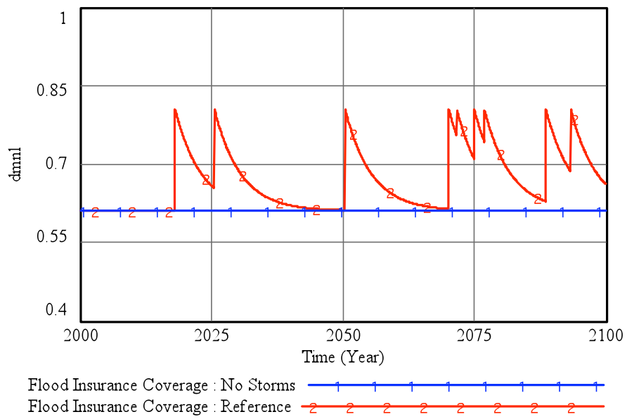
Figure 5-24: The fraction of insurance coverage for the example Reference scenario for Miami-Dade County.
