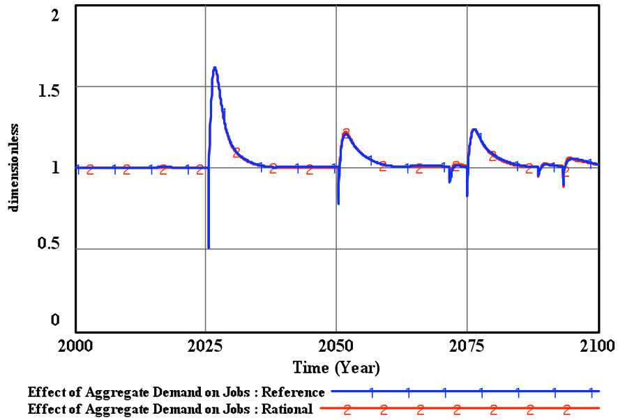
Figure 6-15: The Effect of Aggregate Demand on Jobs for the rationality scenarios (example pattern for Miami-Dade).
