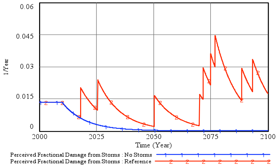
Figure 5-4: The behavior of Perceived Fractional Damage from Storms for the example Reference scenario for Miami-Dade County.
