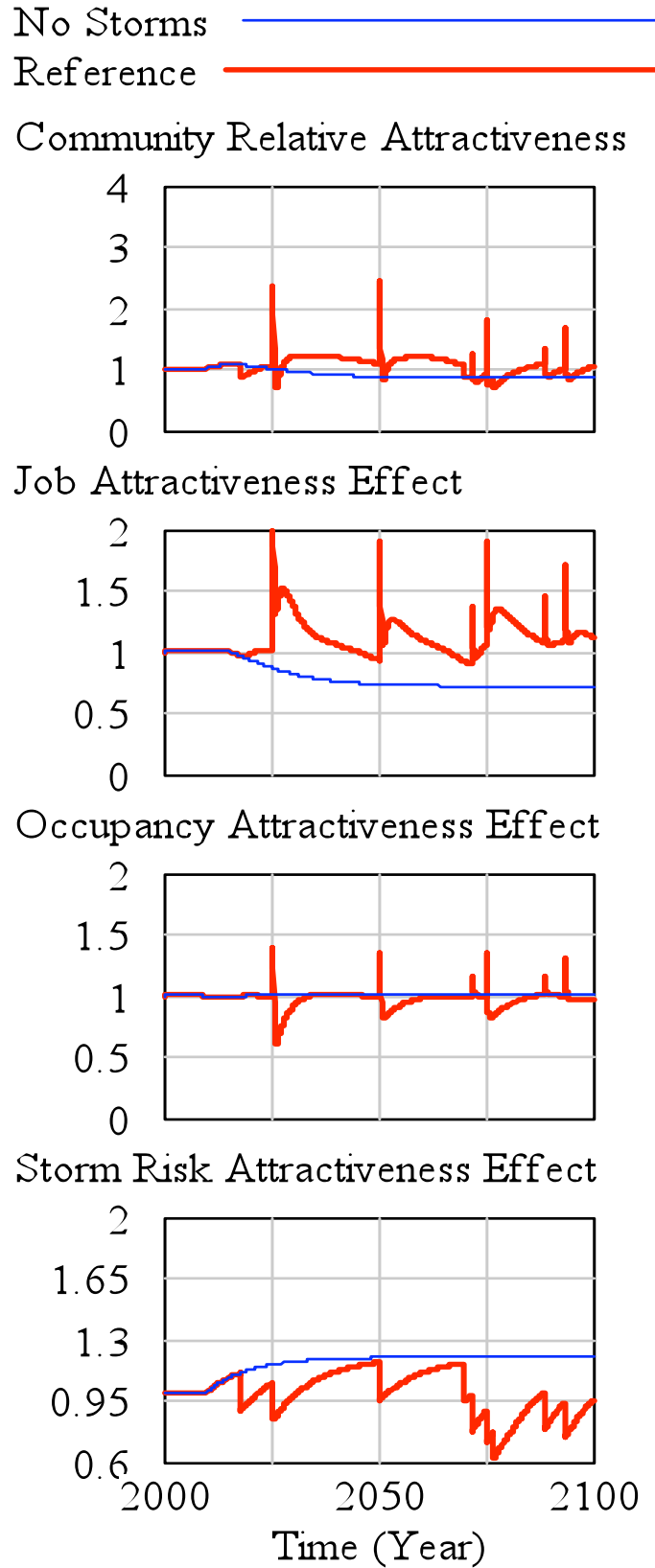
Figure 5-18: Behavior of the three community attractiveness effects for the example Reference scenario for Miami-Dade County.
