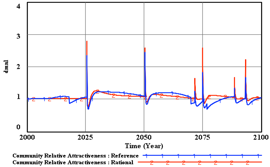
Figure 6-11: The Community Relative Attractiveness for the rationality scenarios (example pattern for Miami-Dade).
