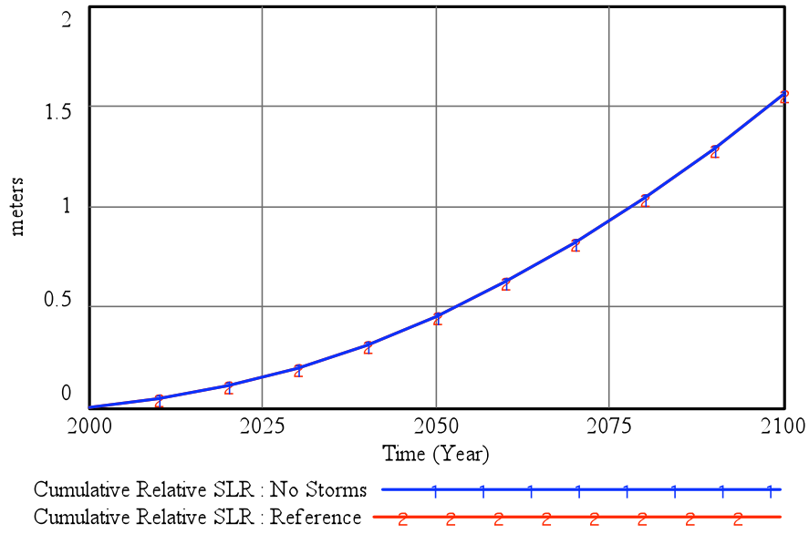
Figure 5-1: Relative SLR results for the example Reference scenario for Miami-Dade County.
