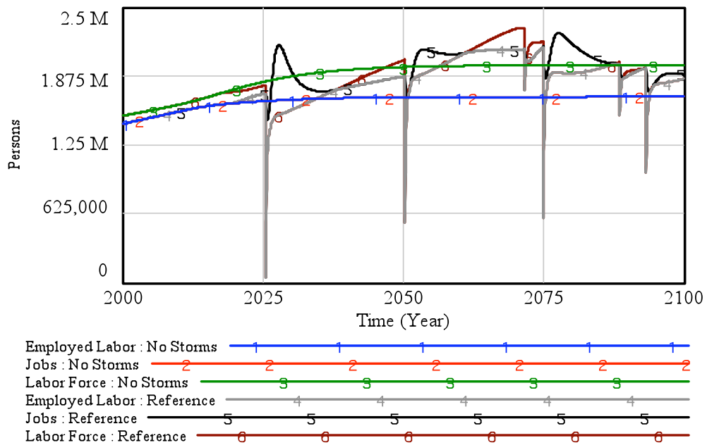
Figure 5-20: The interaction between Labor Force , Jobs , and Employed Labor for the example Reference scenario for Miami-Dade County.
