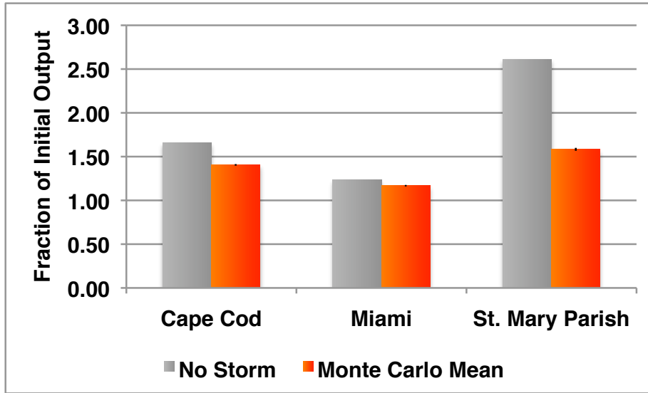
Figure 5-30: Gross Output compared between No Storms and the Monte Carlo means, as a fraction of the initial Gross Output . (Standard errors plotted on Monte Carlo bars, but are small.)
