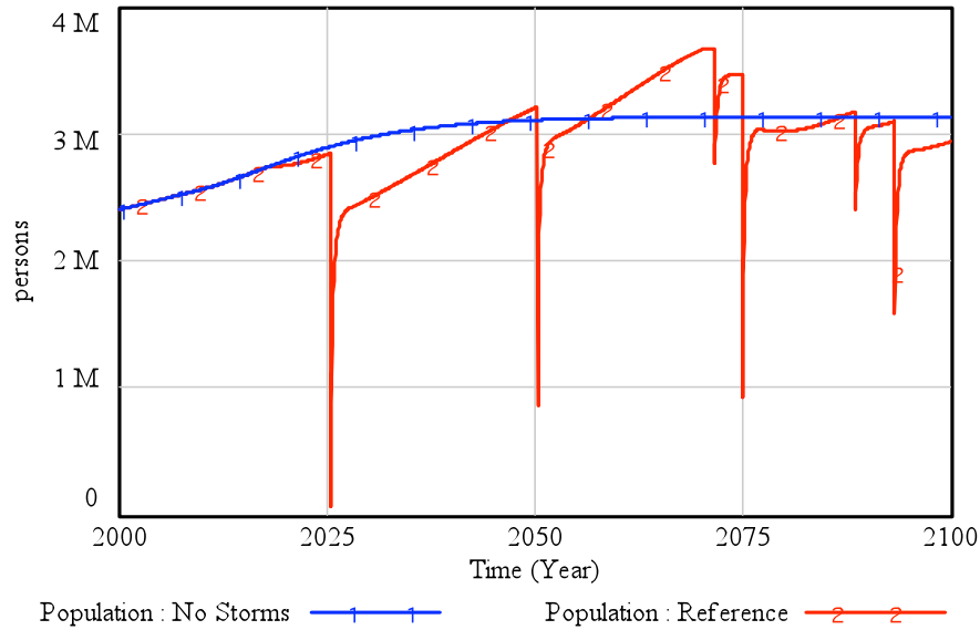
Figure 5-15: Behavior of population for the example Reference scenario for Miami-Dade County.
