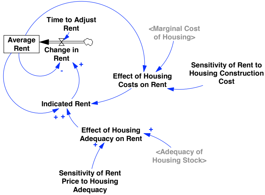
Figure 3-20: Rent price adjustment mechanism.
