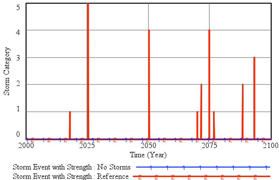
Figure 5-2: The storm pattern for a particular simulation of the Reference scenario, for Miami-Dade County.
