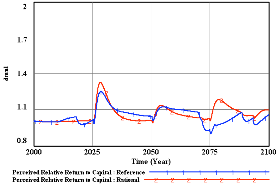
Figure 6-3: The Perceived Relative Return to Capital for the rationality scenarios (example pattern for Miami-Dade).
