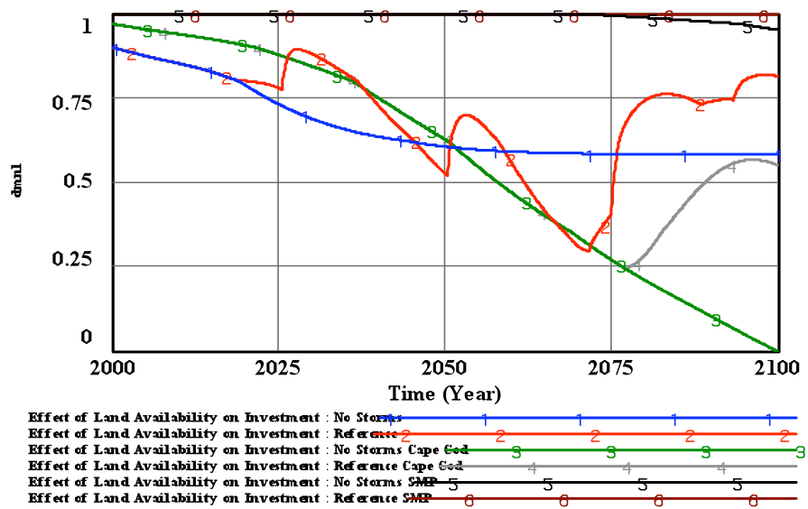
Figure 5-29: The effect of land availability on investment in new infrastructure.
