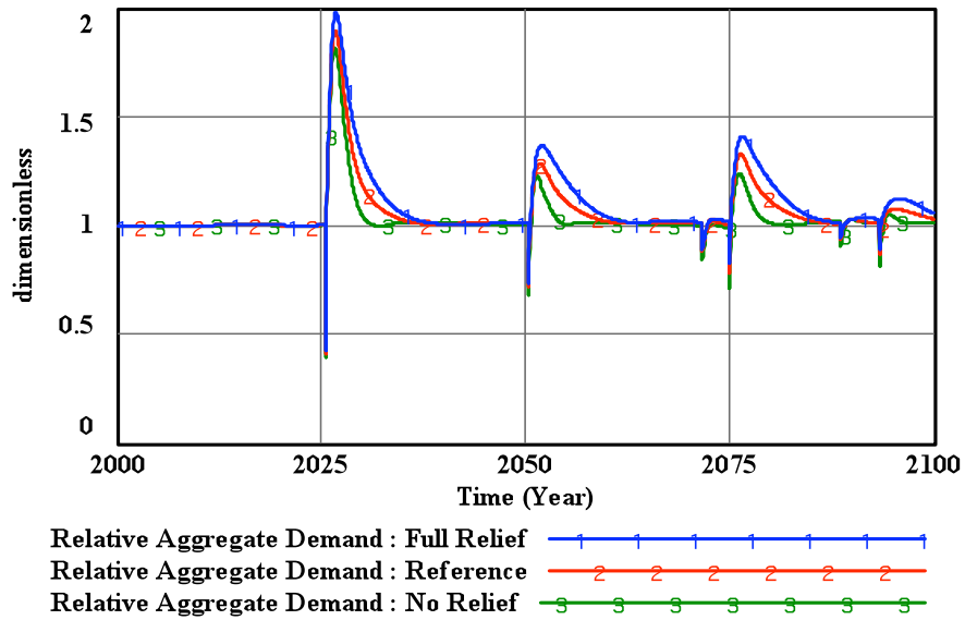
Figure 7-1: Relative Aggregate Demand for the disaster relief scenarios. Behavior is for Miami-Dade County over time, given three different levels of government disaster relief.
