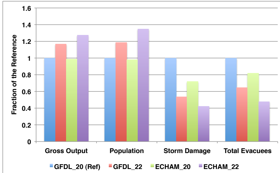
Figure 6-19: Comparison of storm scenarios for Miami-Dade County. Results are normalized to the Monte Carlo mean of Reference scenario.
