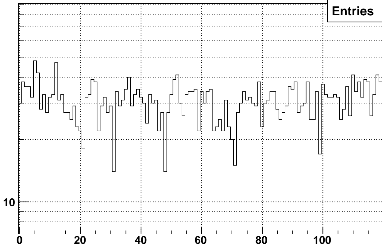
Rate vs. raw bx48 Fill 10448
