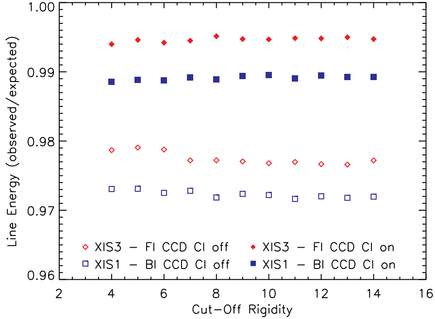
Fig. 10. Fractional change in the XIS line energy as a function of COR, averaging over October-November 2006. Symbols are the same as in Figure 4. A trend toward lower line energy (increased CTI) with higher COR (decreased background) is seen in the FI, charge injection (CI) off data. This results from lower amounts of sacrificial charge. As with the line width in Figure 11, use of charge injection overwhelms the effects of sacrificial charge (solid points).
