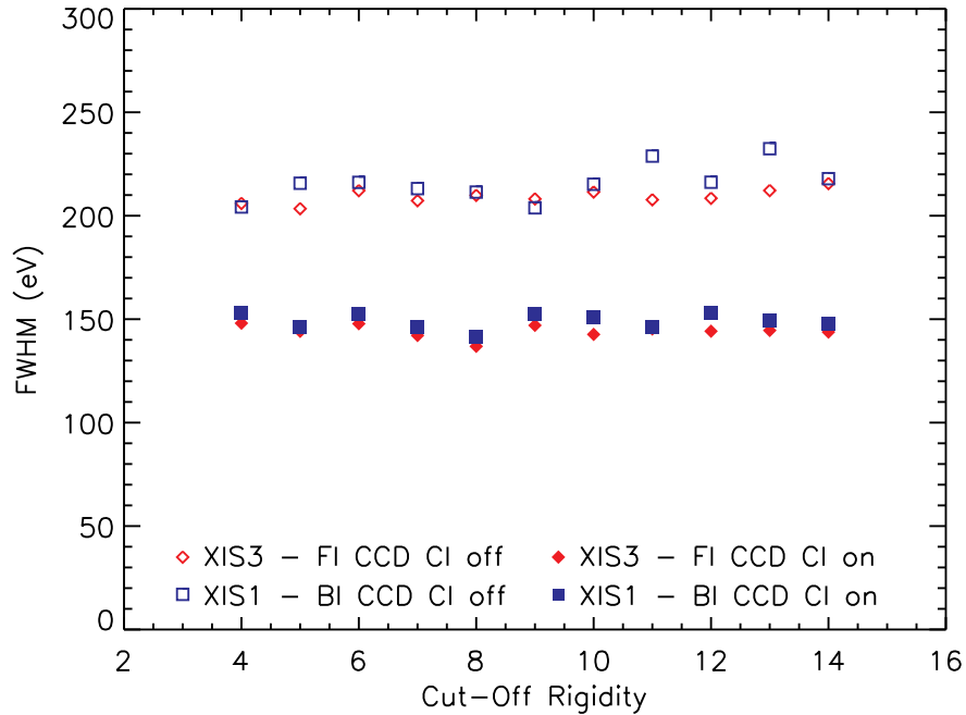
Fig. 11. XIS Mn K\alpha line width (FWHM) as a function of the geomagnetic cut-off rigidity (COR), averaging over October-November 2006. Symbols are the same as in Figure 7. Lower cut-off rigidity indicates a higher particle background, therefore the narrower line widths at low COR in the FI, charge injection (CI) off data (open points) are due to sacrificial charge. Use of charge injection overwhelms the effects of sacrificial charge, so no dependence on COR is seen in those data (solid points).
