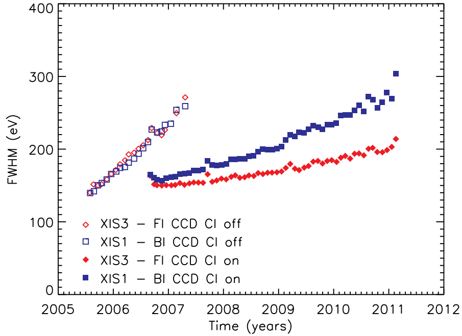
Fig. 8. Change in XIS line width (FWHM) with time over the course of the Suzaku mission, as measured at Mn K\alpha . Different symbols show FI and BI devices with charge injection (CI) on and off.
