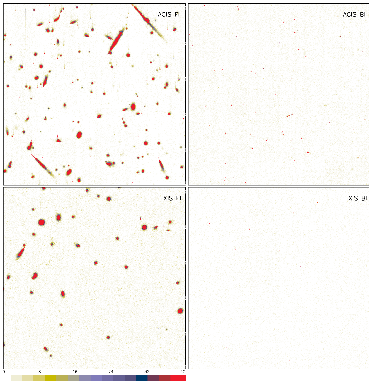
Fig. 10. Raw frame images for ACIS (top) and XIS (bottom), showing an FI (left) and BI (right) device for each. The colorbar shows the pixel values in ADU. An X-ray event from ^{55}\text{Fe} would have a pulseheight around 1500 ADU. The differences between the FI and BI CCDs, and between ACIS and XIS are explained in the text.
