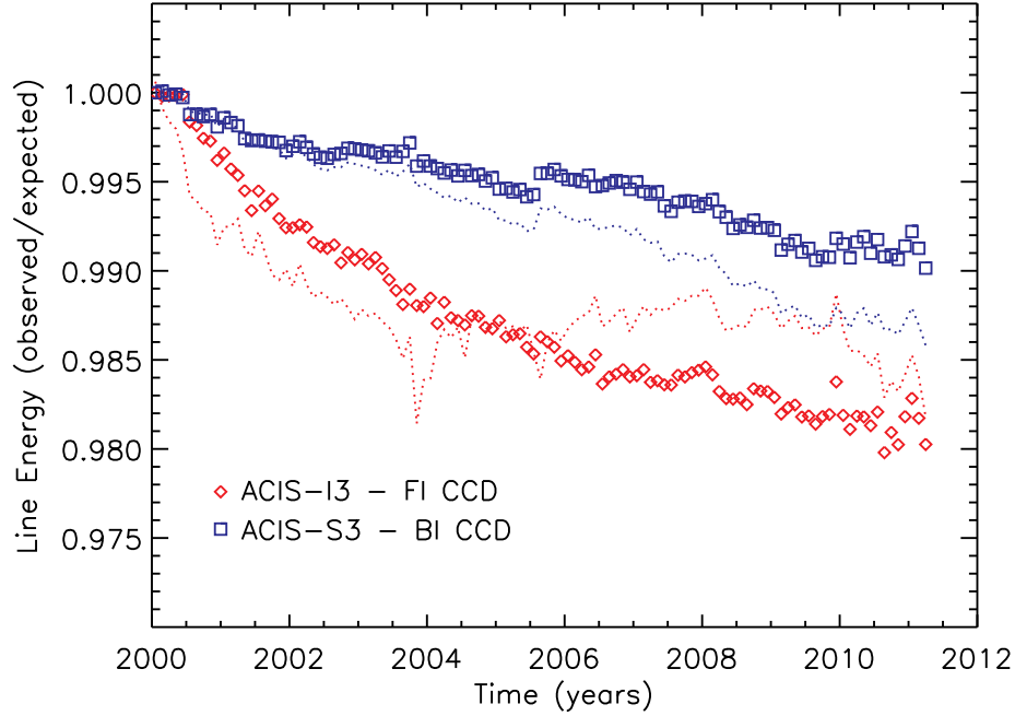
Fig. 13. Fractional change in ACIS line central energy over the course of the Chandra mission, after correcting for sacrificial charge from the particle background. For comparison, the dotted lines show the uncorrected line energy as in Figure 8.
