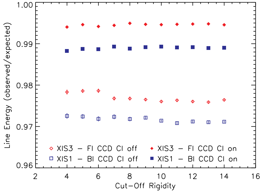
Fig. 14. Fractional change in the XIS line energy as a function of geomagnetic cut-off rigidity (COR), averaging over October-November 2006. Symbols are the same as in Figure 7. Without charge injection, there is a weak dependence of line energy with COR, with higher line energy associated with lower COR, as is expected for sacrificial charge. The use of charge injection overwhelms the effects of sacrificial charge from the particle background (solid symbols). The 1\text{-}\sigma error bars are shown but are often smaller than the symbol sizes.
