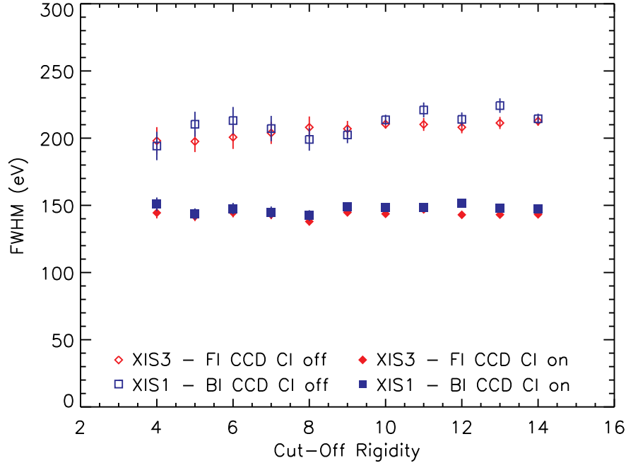
Fig. 15. XIS Mn K\alpha line width (FWHM) as a function of COR, averaging over October–November 2006. Symbols are the same as in Figure 10. Lower cut-off rigidity indicates a higher particle background, therefore the narrower line widths at low COR in the absence of charge injection (open symbols) are due to sacrificial charge. Use of charge injection overwhelms the effects of sacrificial charge, so no dependence on COR is seen in those data (solid symbols).
