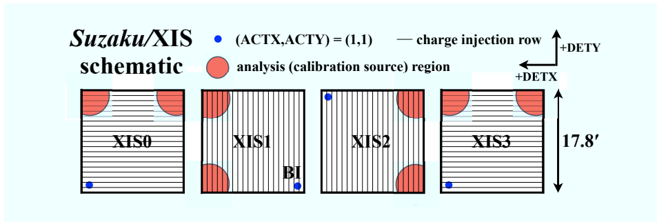
Fig. 2. Schematic drawing of the XIS focal plane. The orange circles show the regions illuminated by the Fe-55 sources. The light grey lines indicate the direction and spacing of the charge injection rows.
