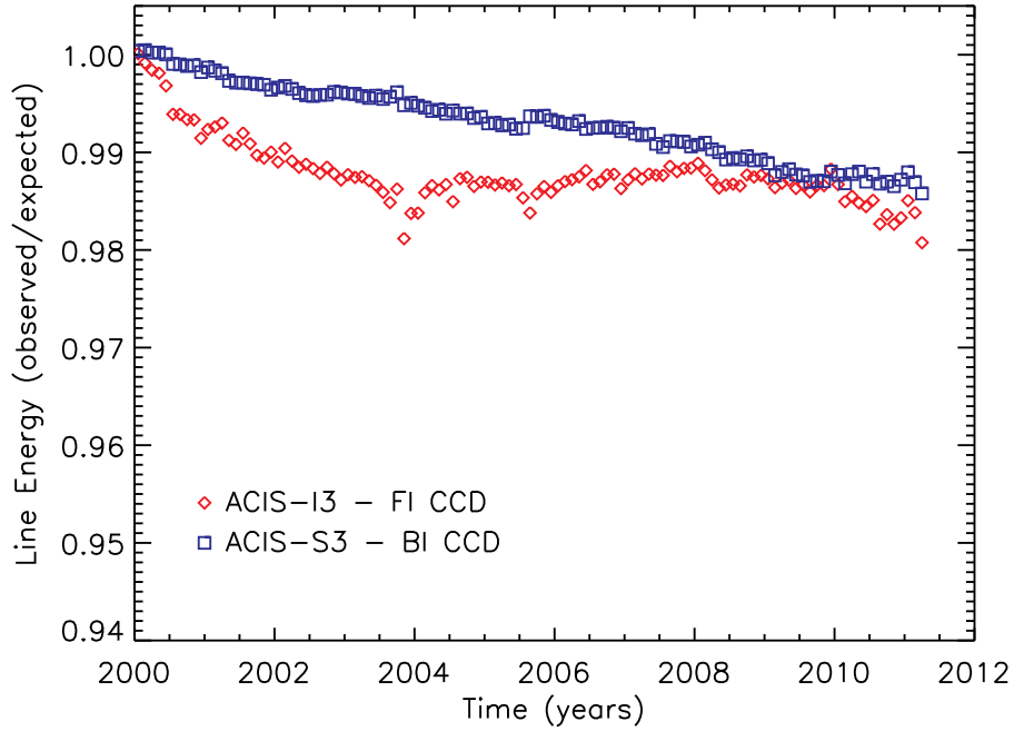
Fig. 9. Fractional change in ACIS line central energy over the course of the Chandra mission, as measured at Mn K\alpha . The effects of varying partial background and sacrificial charge are seen in the ACIS-I3 (FI) data.
