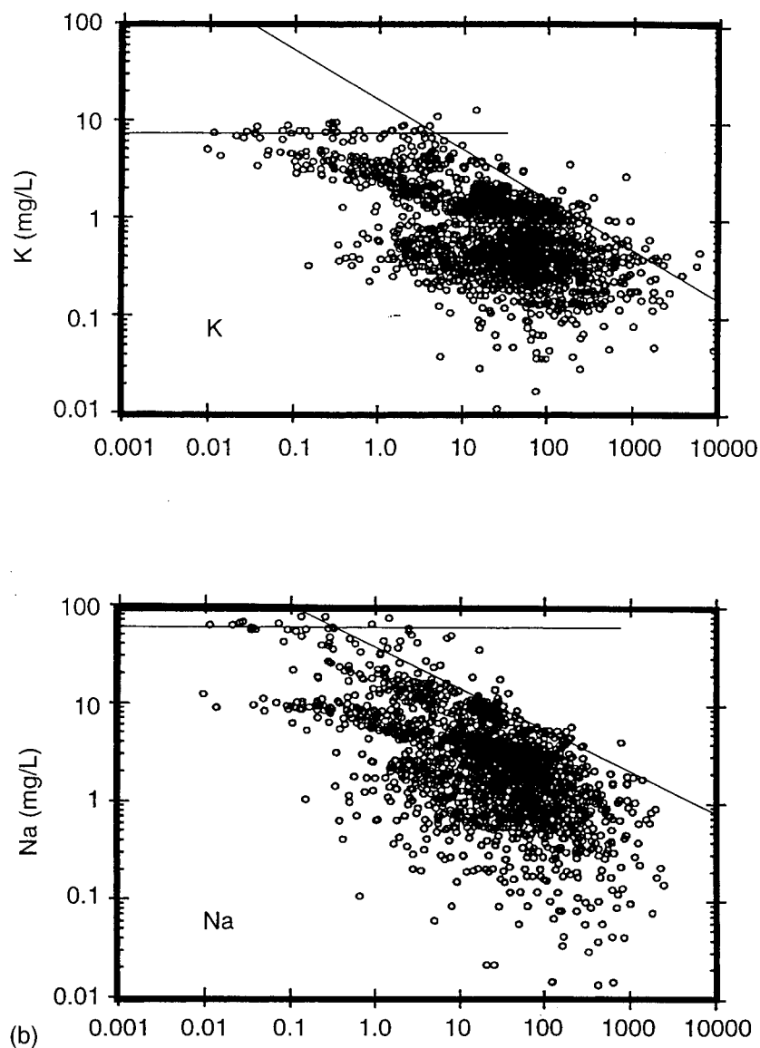
Figure 8 Concentration-discharge relationships for monolithic basalt catchments of the world. Data are shown for Ca, Mg, K, Na, \text{SO}_4 , and total dissolved solids (TDS). Source of data is Bluth (1990).
