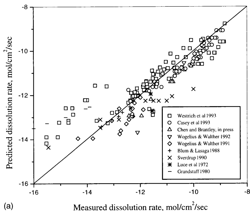
Figure 7 Comparison between observed and model-predicted rates of silicate dissolution. (a) Orthosilicates; (b) Pyroxene; (c) Amphibole.
